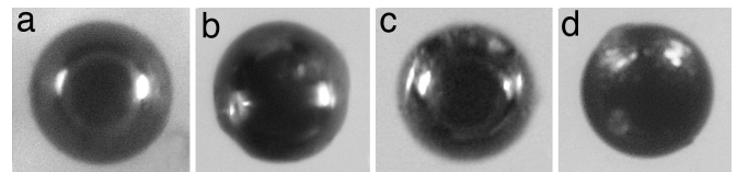
Fig. 2. High-titanomagnetite microspherules from Blackwater Draw, NM (120 \mu\text{m} ) (a); Chobot, AB, Canada (150 \mu\text{m} ) (b), Gainey, MI (90 \mu\text{m} ) (c), and Howard Bay, NC (100 \mu\text{m} ) (d).
